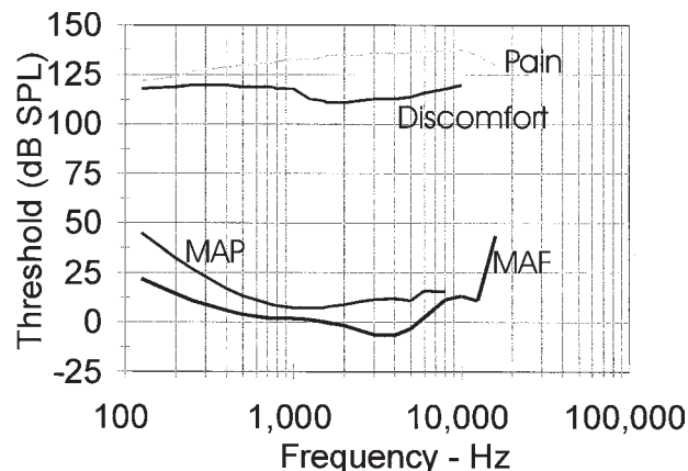
Figure 5.10 The thresholds of hearing in decibels of sound pressure level (dB SPL) are shown as a function of frequency for Minimal Audible Field (MAF) thresholds, MAP, thresholds for pain, and thresholds for discomfort. The thresholds for pain and discomfort represent estimates of the upper limit of level that humans can tolerate. Source: These thresholds are based on national and international standards.
